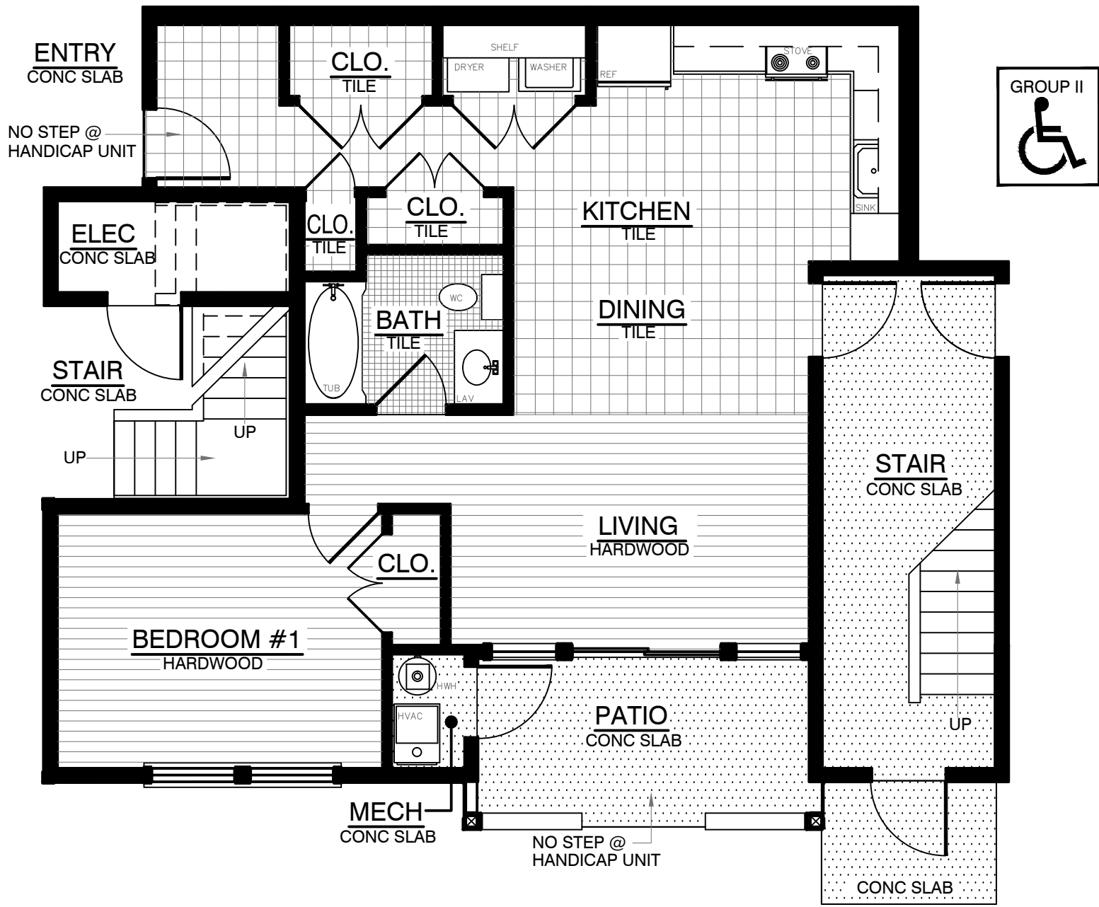
TYPICAL (1) BEDROOM - HANDICAP UNIT (726 SQ. FT.) MARION VILLAGE ESTATES - MARION, MASSACHUSETTS
