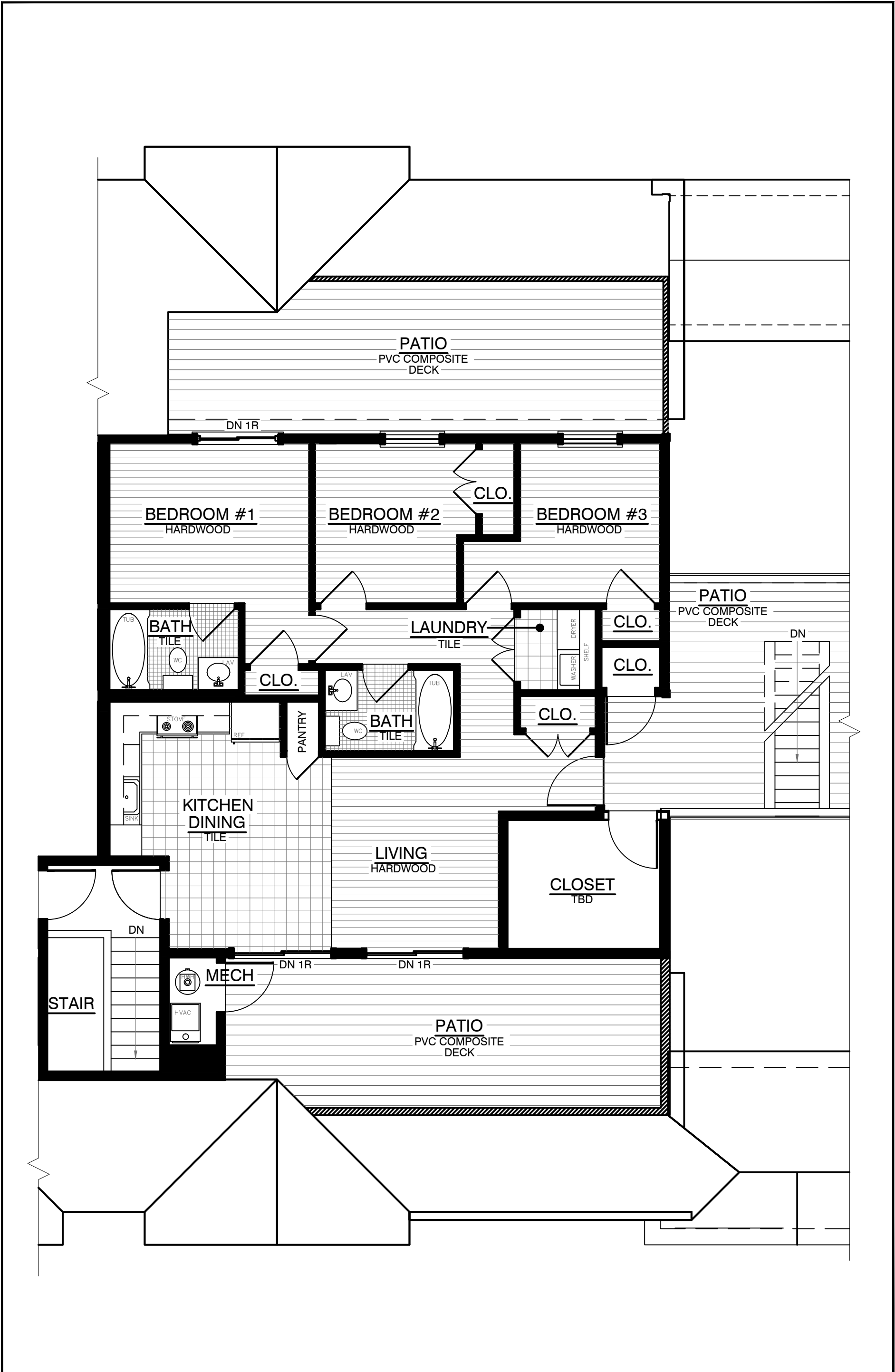
TYPICAL (3) BEDROOM THIRD FLOOR UNIT ( 939 SQ. FT.) MARION VILLAGE ESTATES - MARION, MASSACHUSETTS
